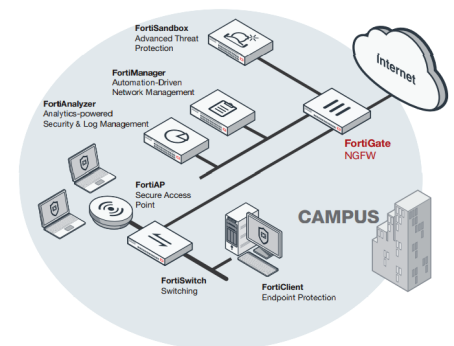
FortiGate 200F deployment in Campus (NGFW)
