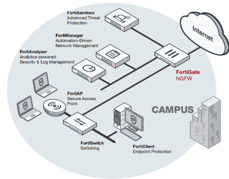
FortiGate 500E deployment in Campus (NGFW)
