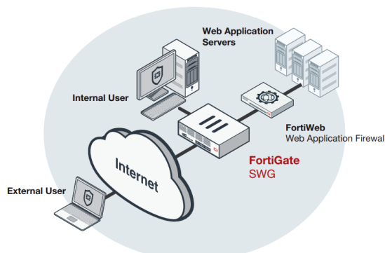
FortiGate 500E SWG deployment
